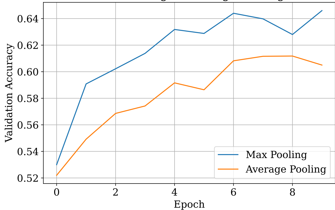
Max Pooling vs Average Pooling
